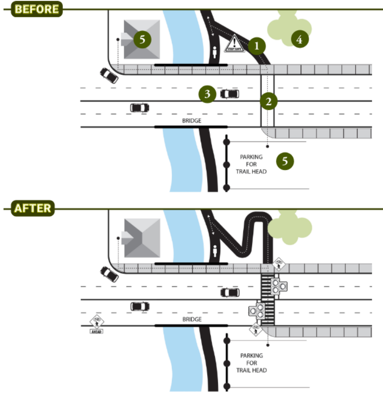
Figure 3: Example trail crossing improvement (FHWA STEP)
